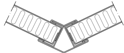
PM-15 Angular corner profile (according to project)
