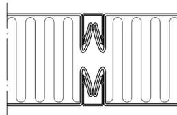
PM-01 Joint panel
