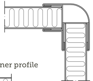
PM-42 Corner profile with curved side
