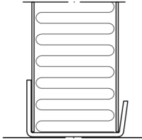
PG-03 50 mm Lower supporting profile
